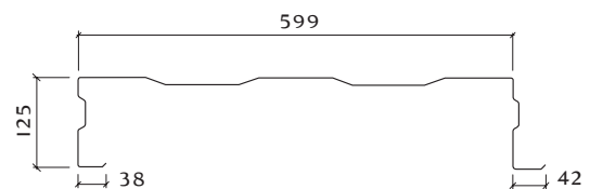
C-kazetta LT125
